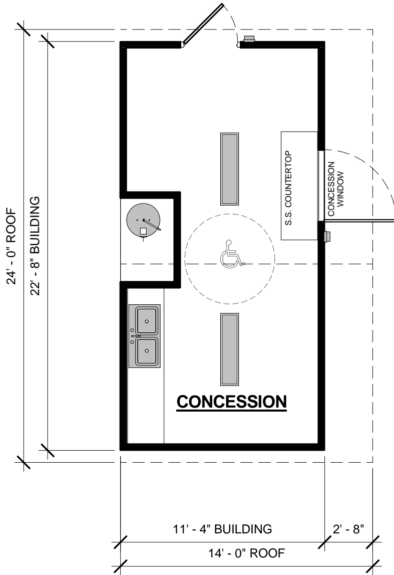
1 FLOOR PLAN 3/16" = 1'-0"
