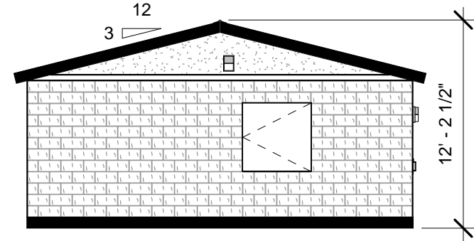
2 FRONT ELEVATION 1/8" = 1'-0"
