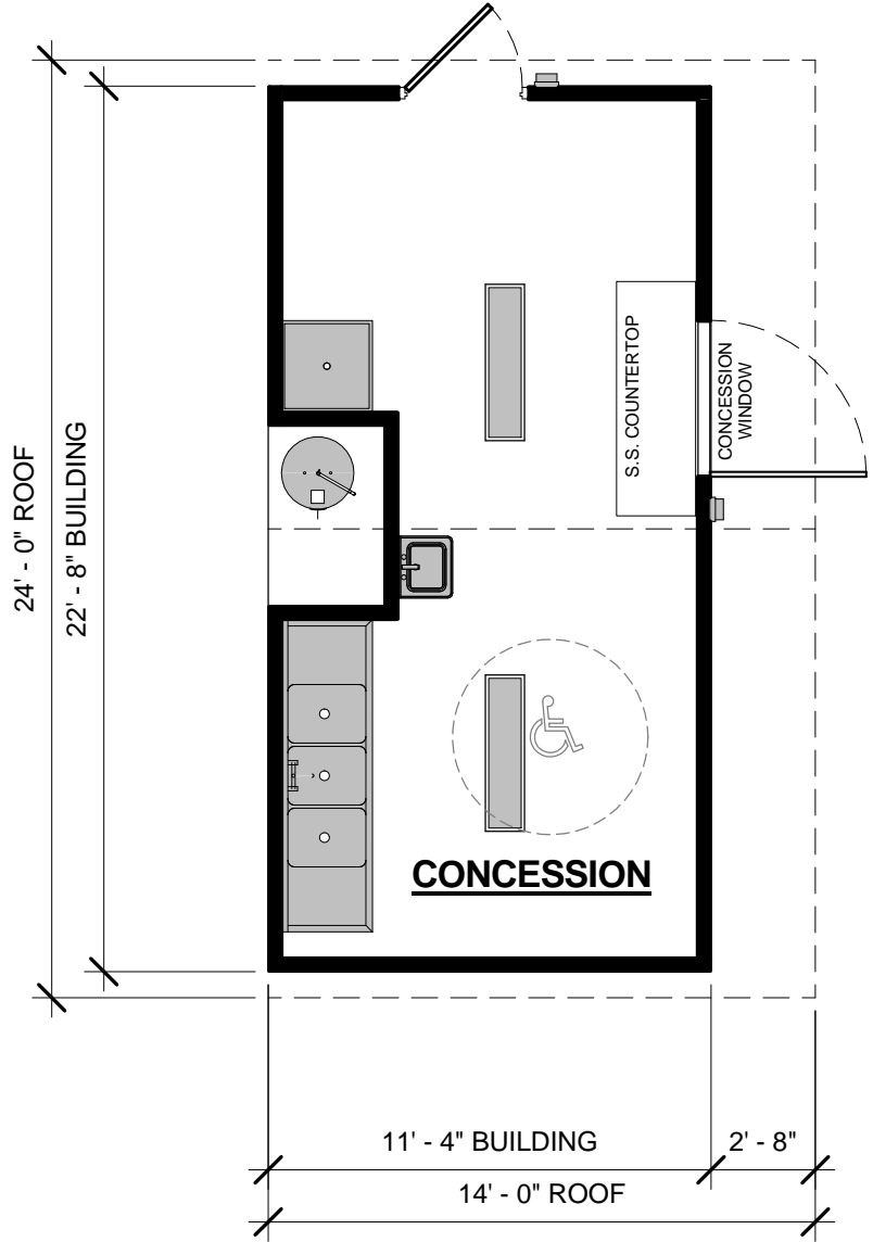
1 FLOOR PLAN 3/16" = 1'-0"
