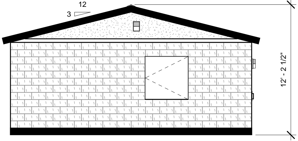
2 FRONT ELEVATION 3/16" = 1'-0"
