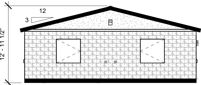
2 FRONT ELEVATION 1/8" = 1'-0"
