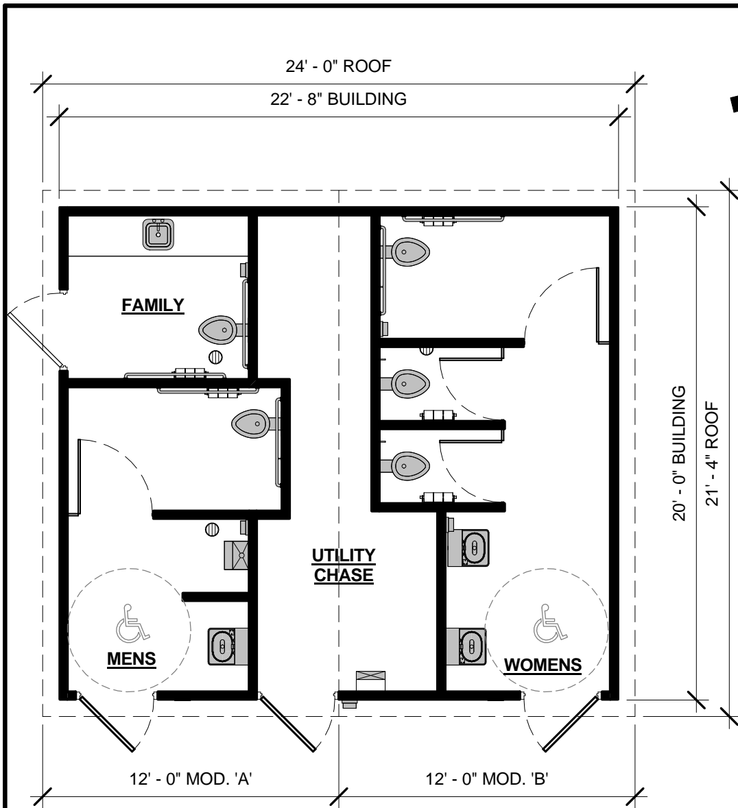
1 FLOOR PLAN 3/16" = 1'-0"
