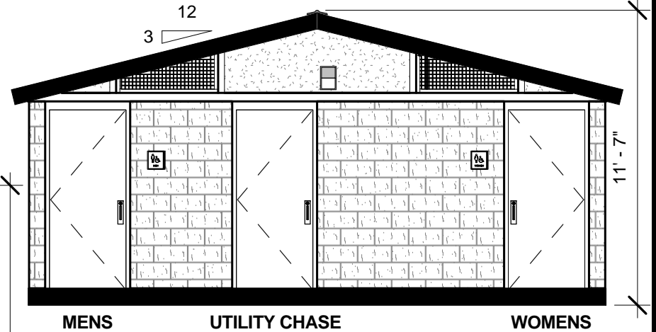
2 FRONT ELEVATION 3/16" = 1'-0"
