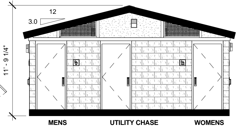
3 RIGHT ELEVATION 3/16" = 1'-0"
