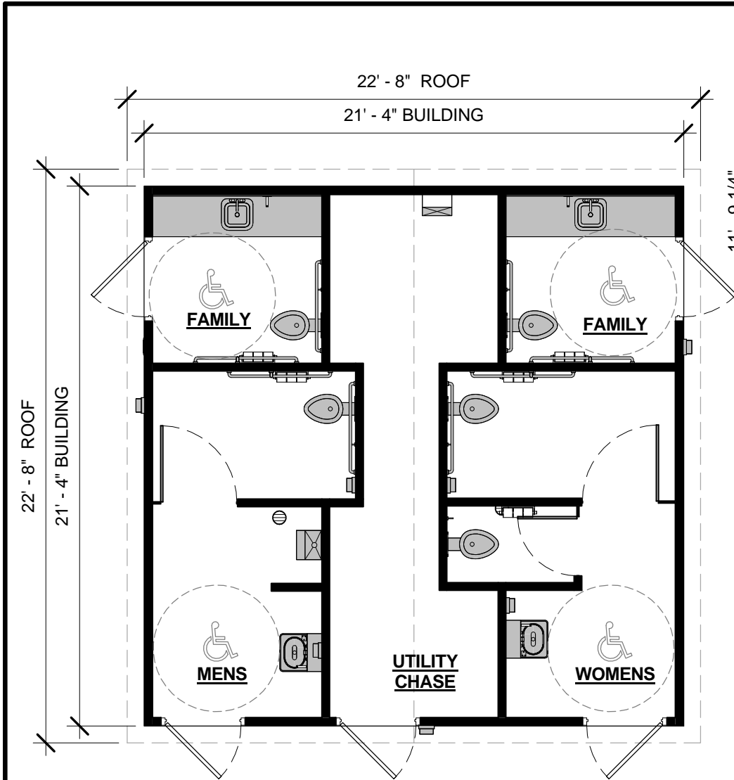
1 FLOOR PLAN 3/16" = 1'-0"
