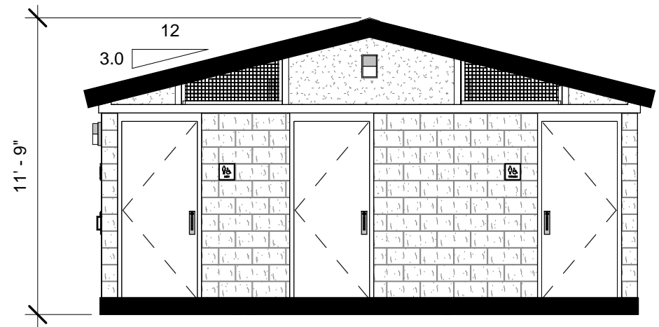
② FRONT ELEVATION 3/16" = 1'-0"
