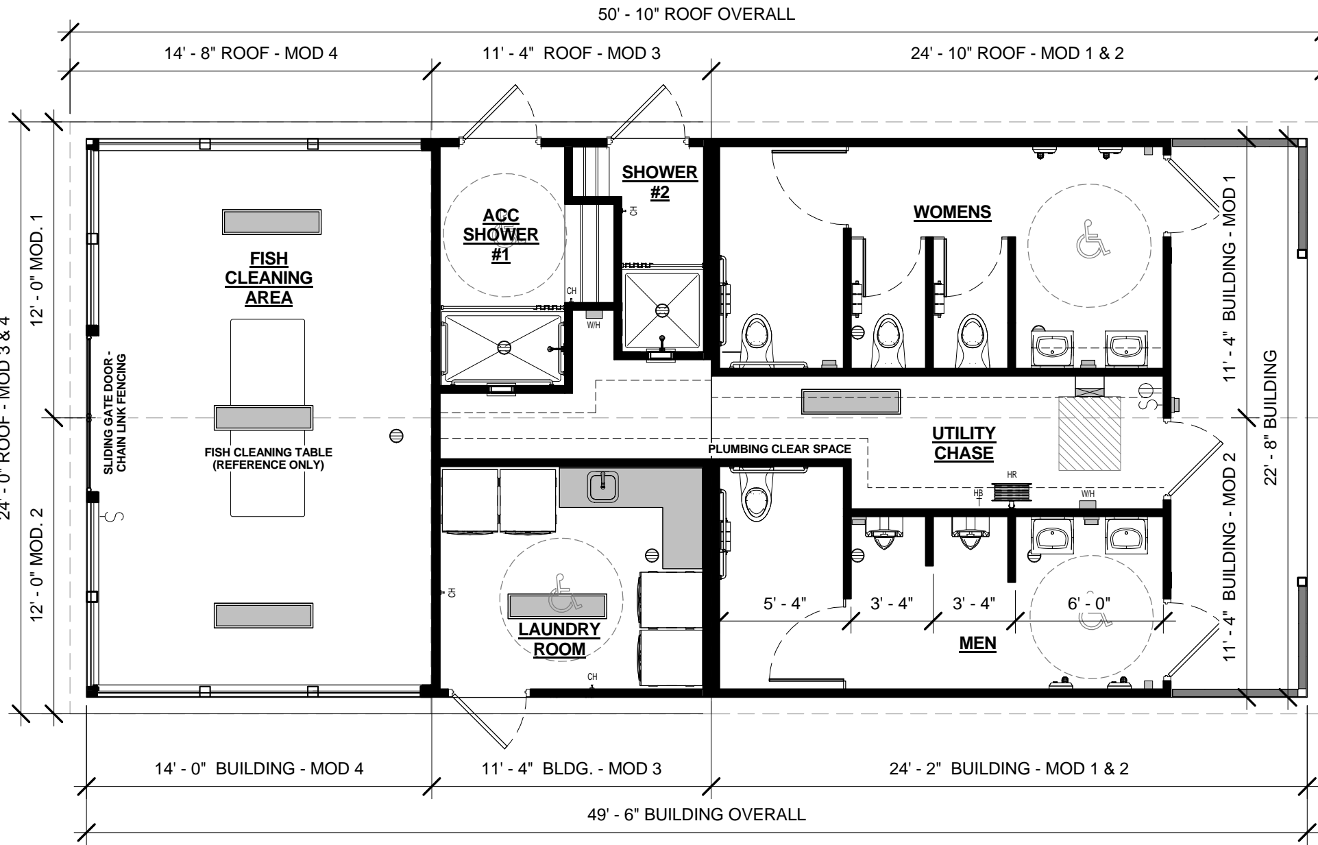
1 FLOOR PLAN 3/16" = 1'-0"
