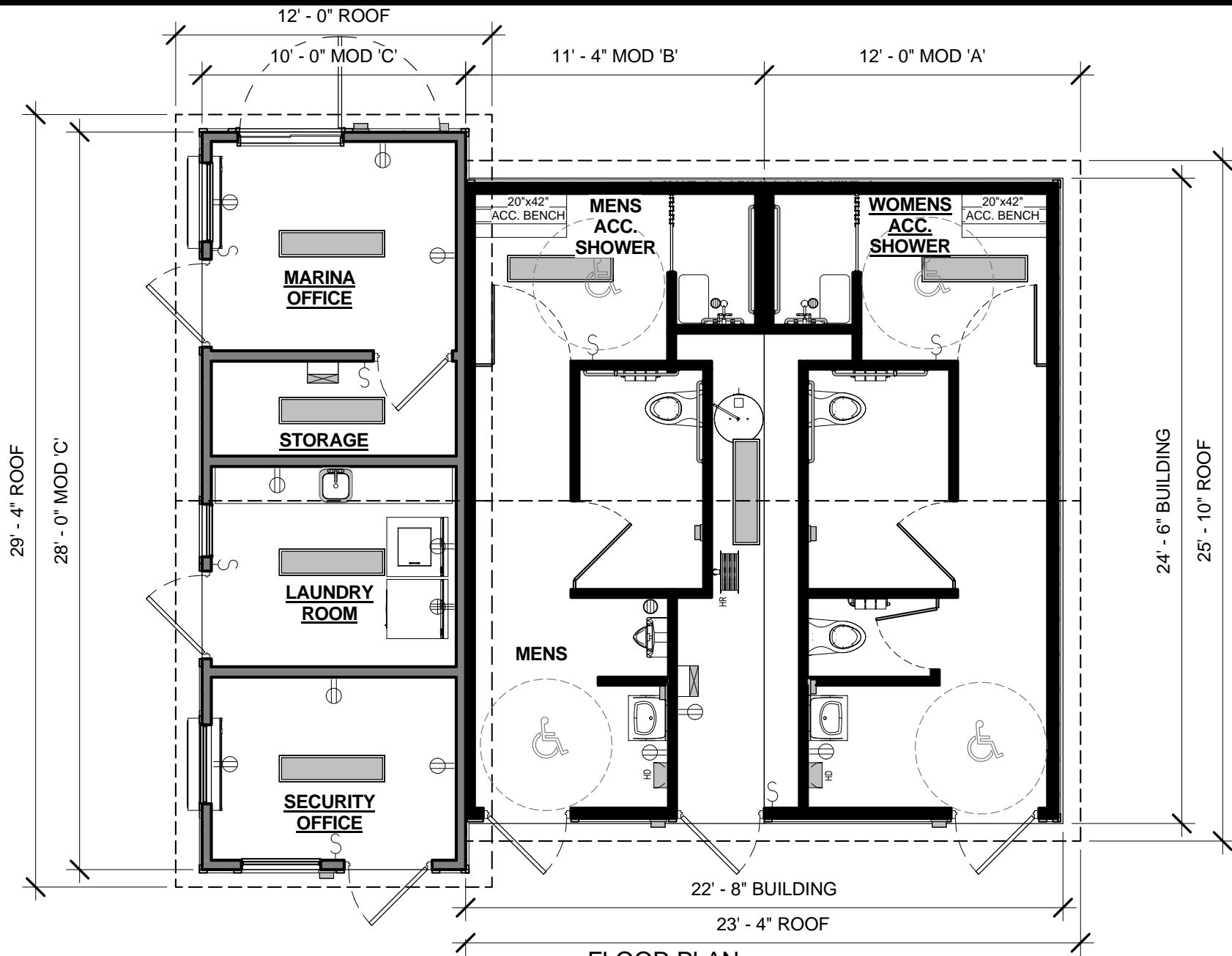
1 FLOOR PLAN 3/16" = 1'-0"
