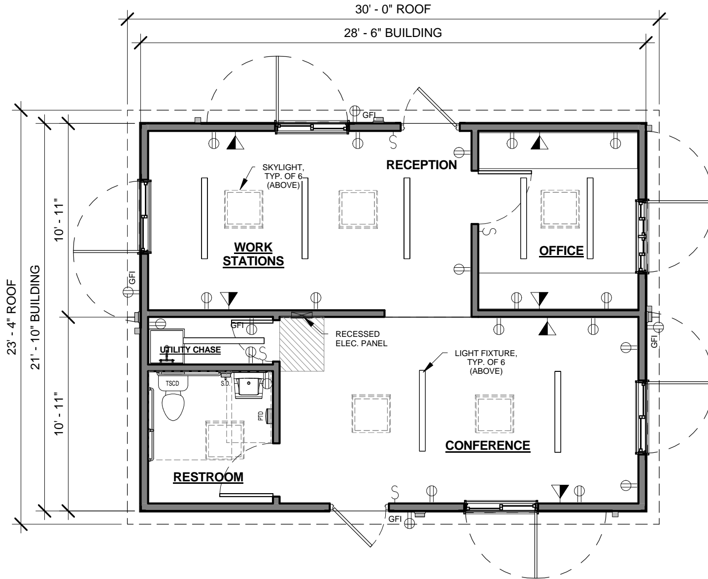
1 FLOOR PLAN 3/16" = 1'-0"
