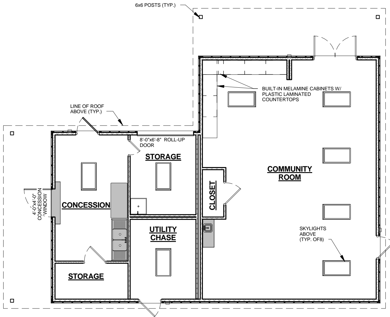
1 FLOOR PLAN 1/8" = 1'-0"
