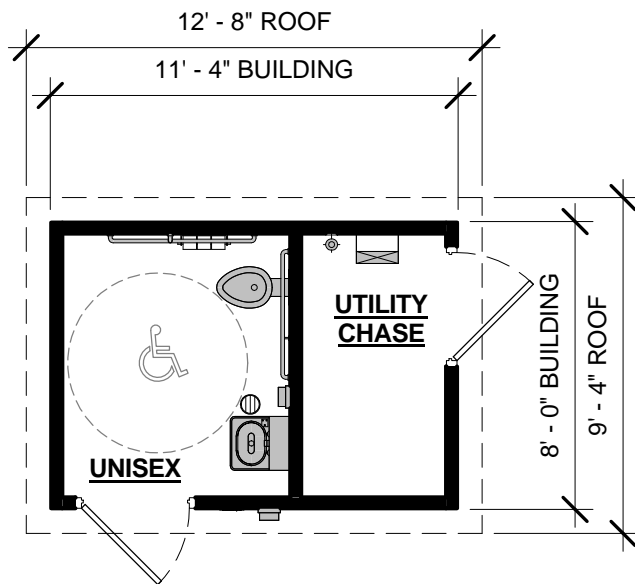
1 FLOOR PLAN 3/16" = 1'-0"
