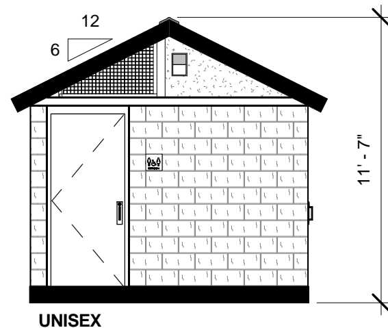
2 FRONT ELEVATION 3/16" = 1'-0"
