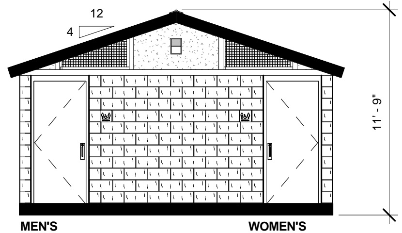
2 FRONT ELEVATION 3/16" = 1'-0"
