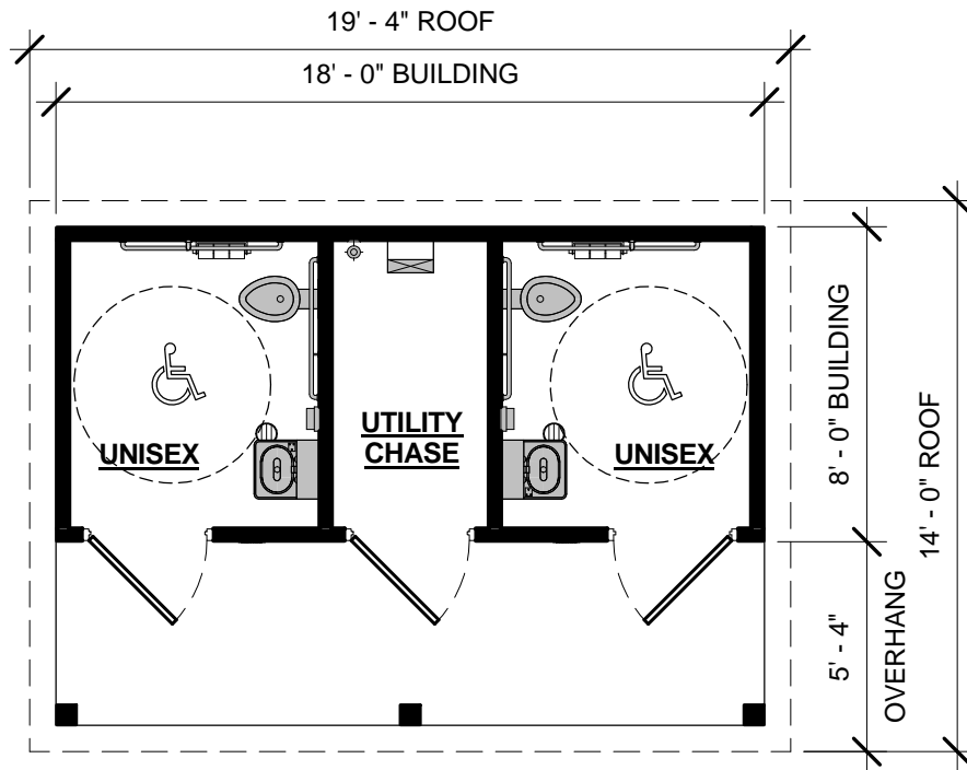
1 FLOOR PLAN 3/16" = 1'-0"
