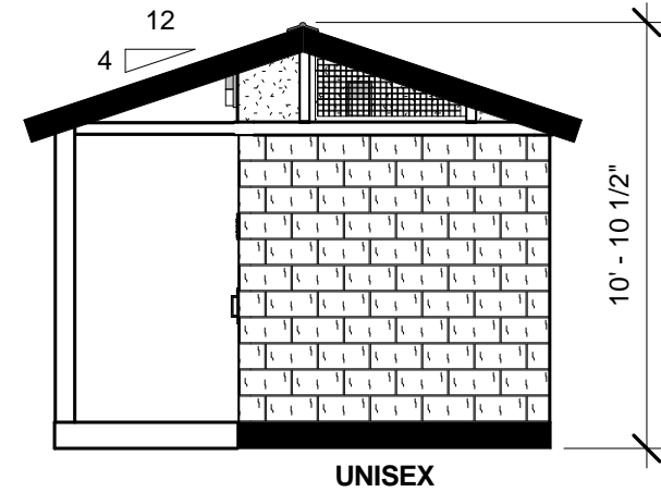
2 RIGHT ELEVATION 3/16" = 1'-0"
