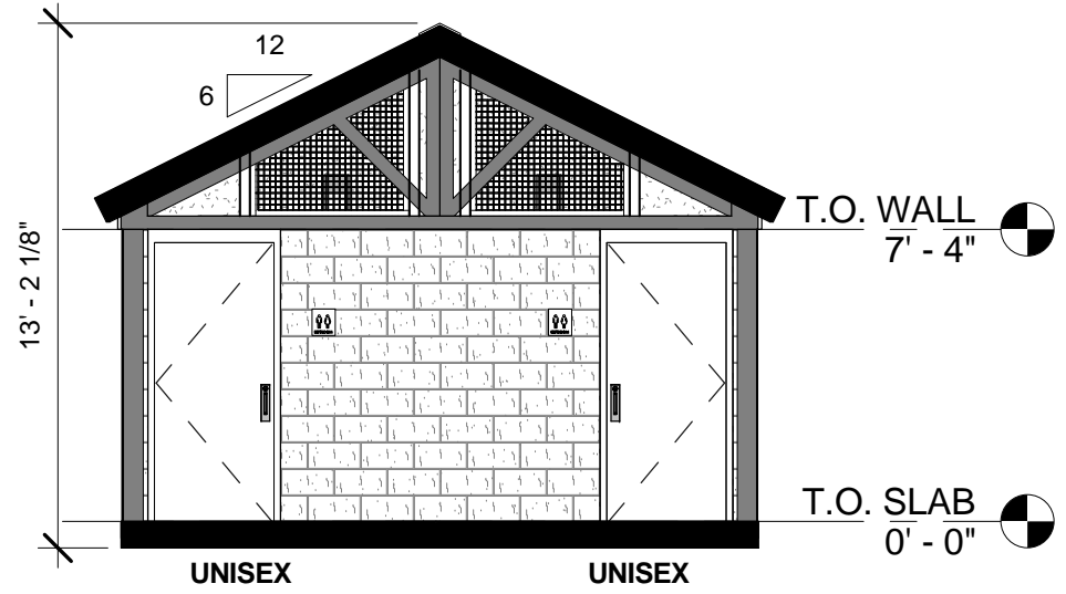
3 FRONT ELEVATION 3/16" = 1'-0"
