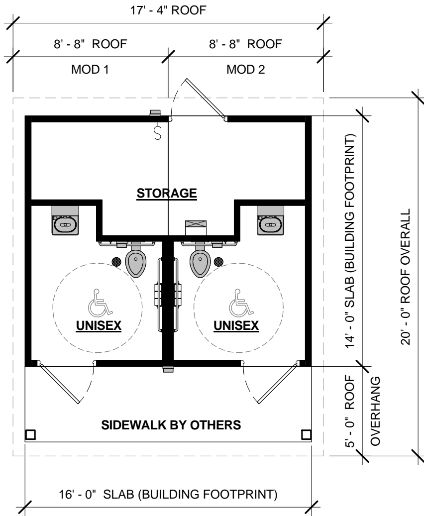
1 FLOOR PLAN 3/16" = 1'-0"
