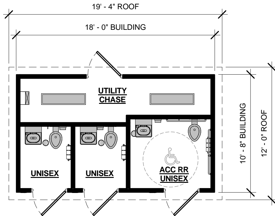
1 FLOOR PLAN 3/16" = 1'-0"
