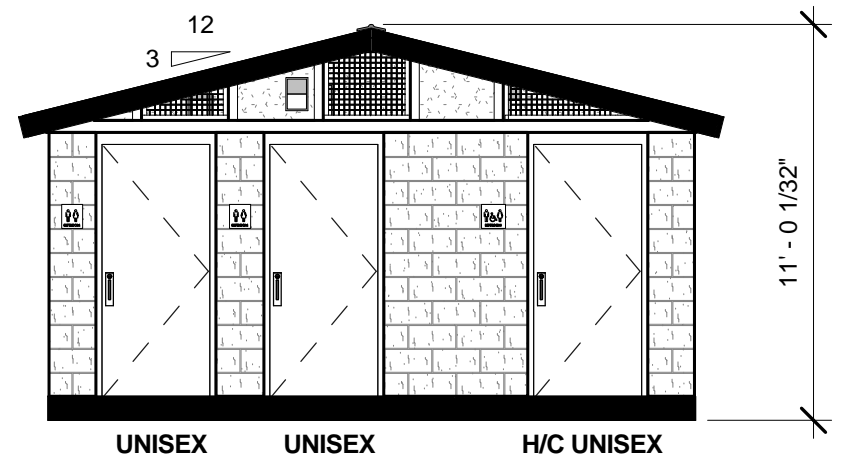
2 FRONT ELEVATION 3/16" = 1'-0"
