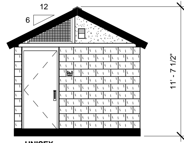
UNISEX 2 FRONT ELEVATION 3/16" = 1'-0"
