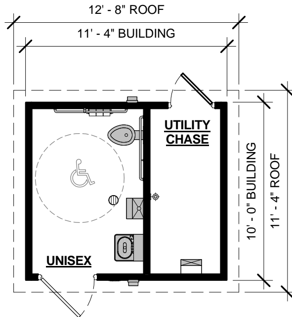
1 FLOOR PLAN 3/16" = 1'-0"
