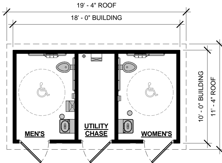
1 FLOOR PLAN 3/16" = 1'-0"
