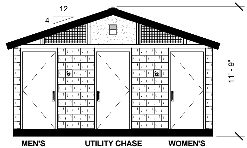
2 FRONT ELEVATION 3/16" = 1'-0"
