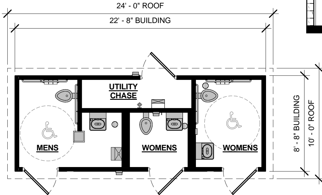
1 FLOOR PLAN 3/16" = 1'-0"
