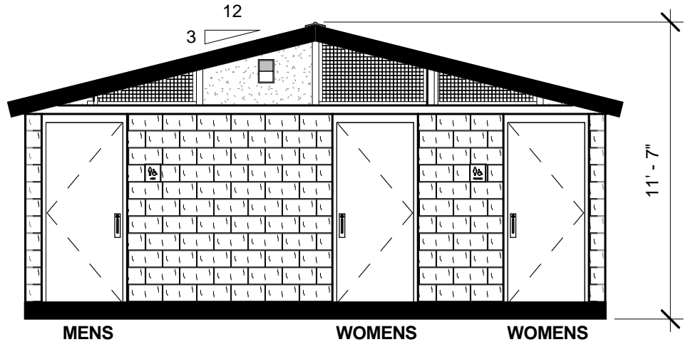
2 FRONT ELEVATION 3/16" = 1'-0"
