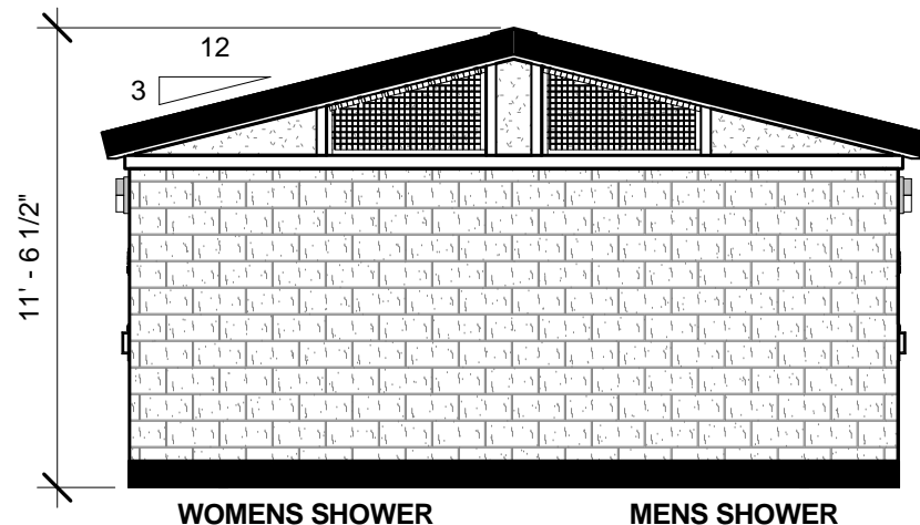
2 FRONT ELEVATION 3/16" = 1'-0"
