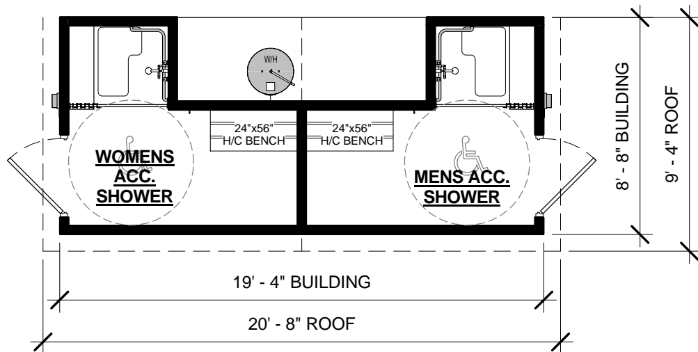
1 FLOOR PLAN 3/16" = 1'-0"
