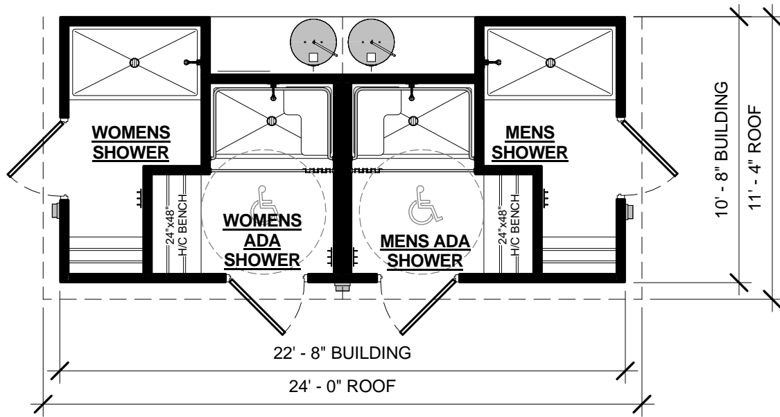
① FLOOR PLAN 3/16" = 1'-0"
