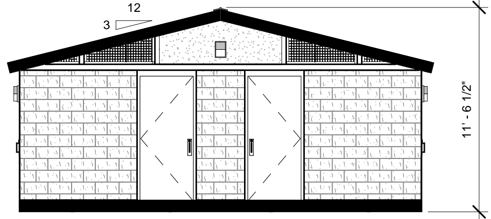
② FRONT ELEVATION 3/16" = 1'-0"
