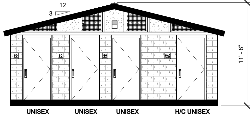
2 FRONT ELEVATION 3/16" = 1'-0"
