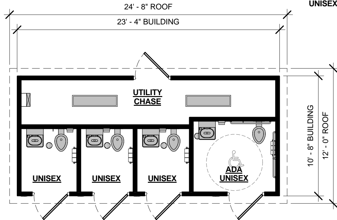
1 FLOOR PLAN 3/16" = 1'-0"
