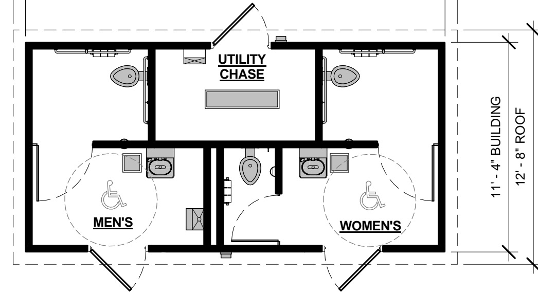
1 FLOOR PLAN 3/16" = 1'-0"
