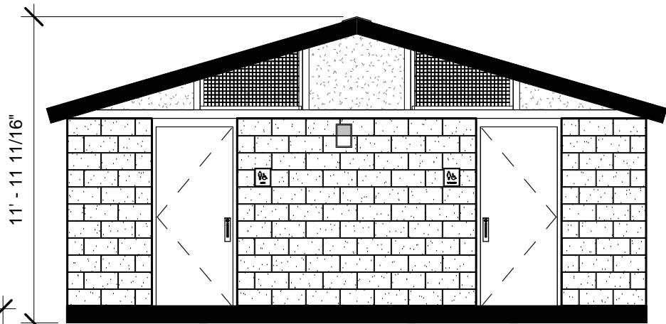
2 FRONT ELEVATION 3/16" = 1'-0"
