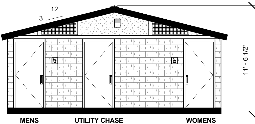
2 FRONT ELEVATION 3/16" = 1'-0"
