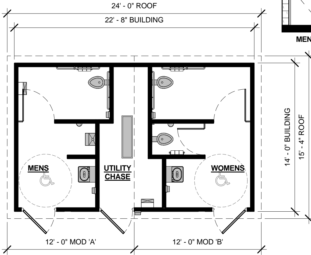
1 FLOOR PLAN 3/16" = 1'-0"
