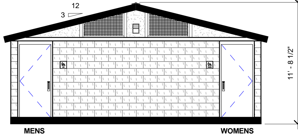
2 FRONT ELEVATION 3/16" = 1'-0"
