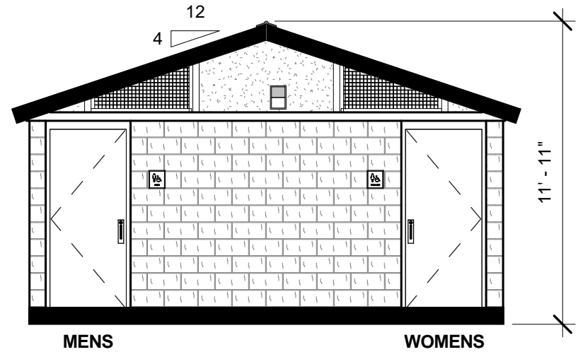
2 FRONT ELEVATION 3/16" = 1'-0"
