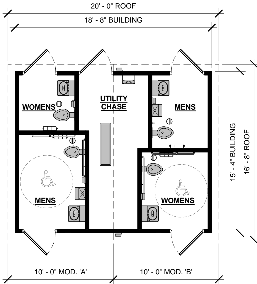
1 FLOOR PLAN 3/16" = 1'-0"
