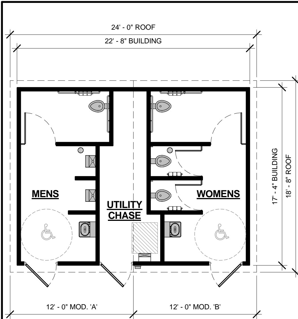
1 FLOOR PLAN 3/16" = 1'-0"
