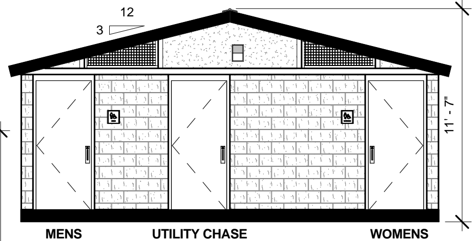
2 FRONT ELEVATION 3/16" = 1'-0"
