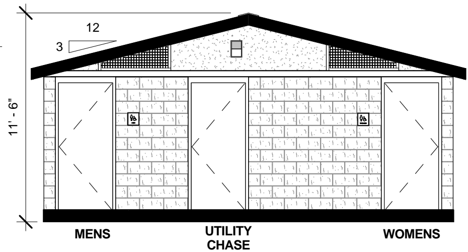
3 FRONT ELEVATION 3/16" = 1'-0"
