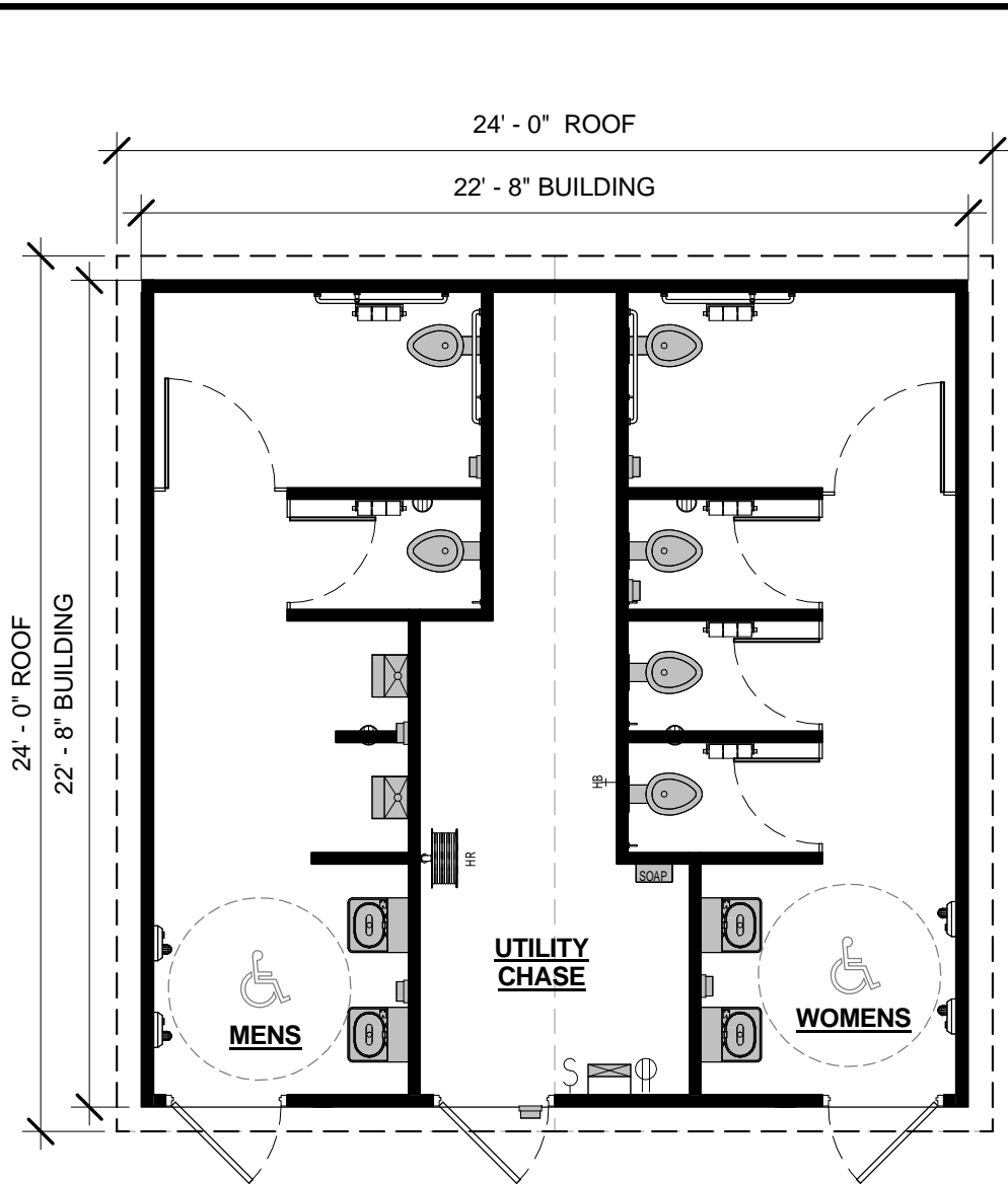
1 FLOOR PLAN 3/16" = 1'-0"
