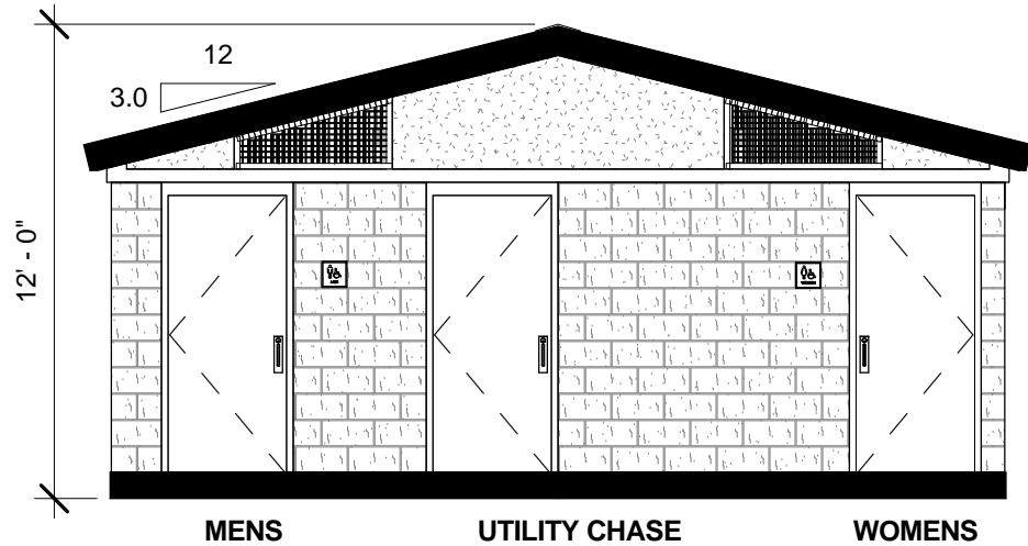
3 FRONT ELEVATION 3/16" = 1'-0"
