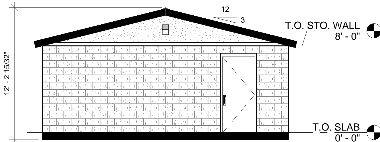
2 FRONT ELEVATION 3/16" = 1'-0"
