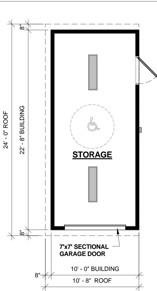
1 FLOOR PLAN 3/16" = 1'-0"
