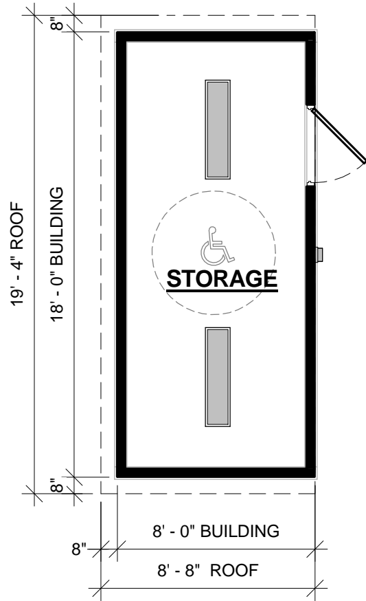
① FLOOR PLAN 3/16" = 1'-0"
