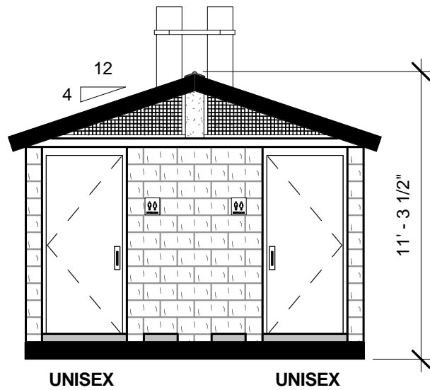
2 FRONT ELEVATION 3/16" = 1'-0"
