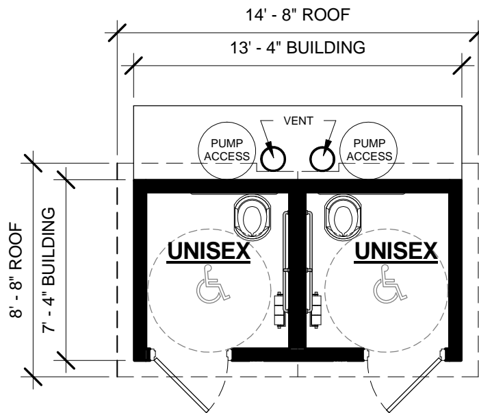
1 FLOOR PLAN 3/16" = 1'-0"
