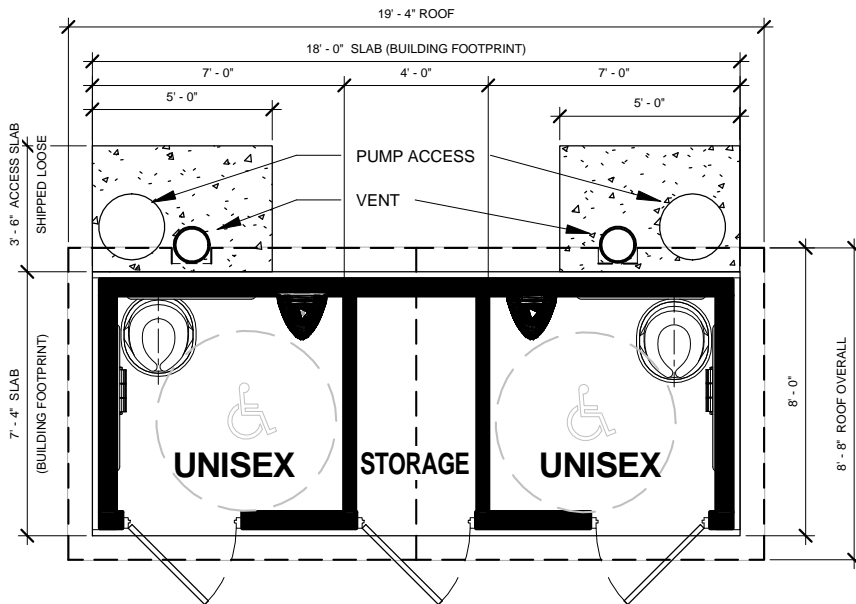
1 FLOOR PLAN 3/16" = 1'-0"
