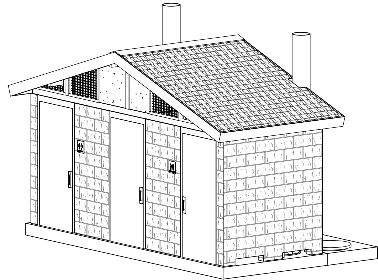
3 PERSPECTIVE
