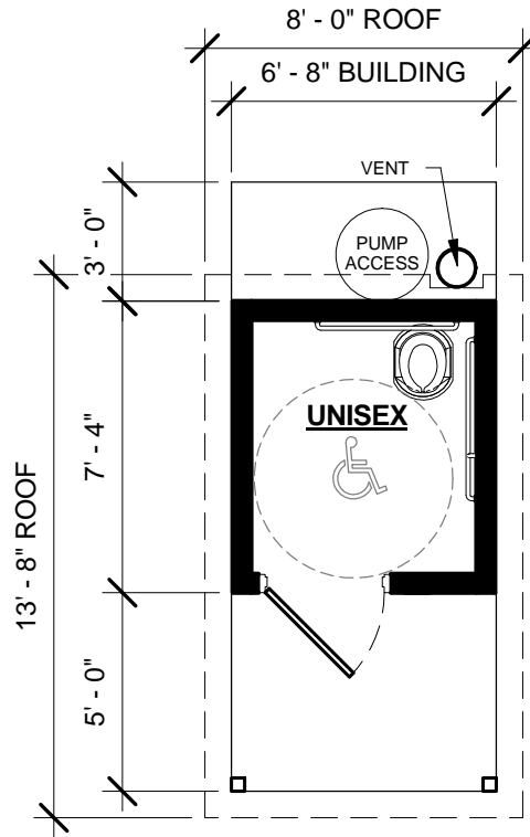
① FLOOR PLAN 3/16" = 1'-0"
