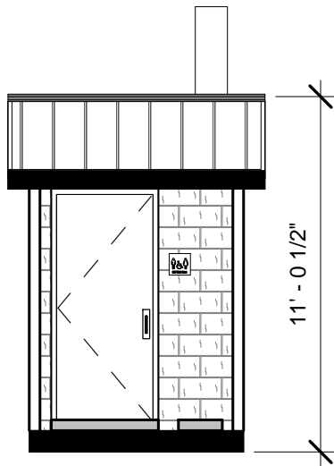
② FRONT ELEVATION 3/16" = 1'-0"
