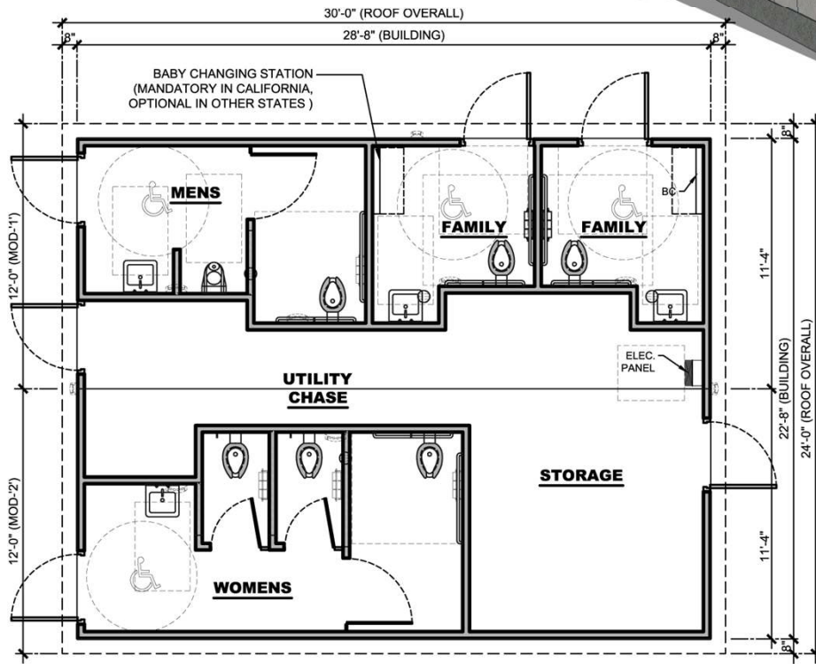
FLOOR PLAN
