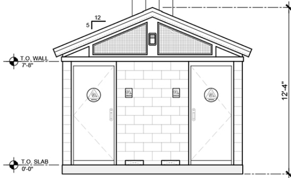
ELEVATION 1 SCALE: 3/16"=1'-0"
