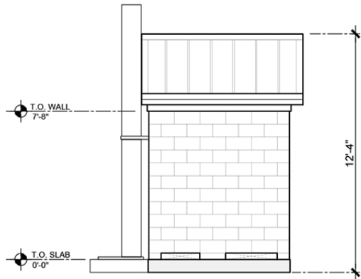
ELEVATION 2 SCALE: 3/16"=1'-0"
