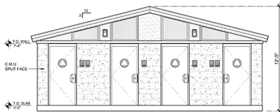
ELEVATION SCALE: NOT TO SCALE
