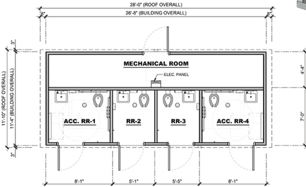
FLOOR PLAN SCALE: NOT TO SCALE
